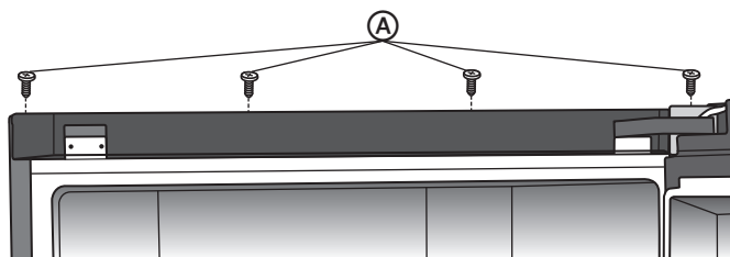
(A) Screws
